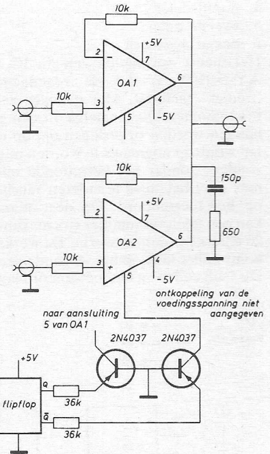
Fig. 8. Multiplexer.
