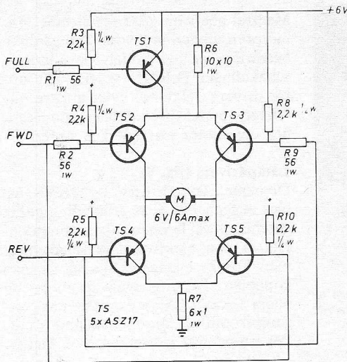
Fig. 6. Motorschakeling.
